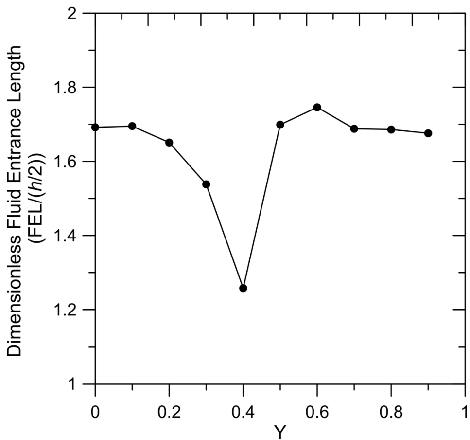
Figure S1 Dimensionless FEL as a function of cross-pore position ( Y )
