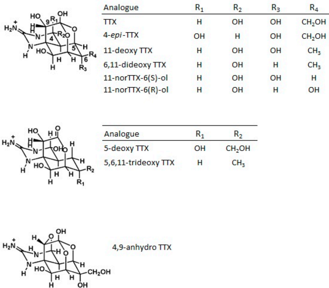
Figure S1. Structures of selected Tetrodotoxin analogues
