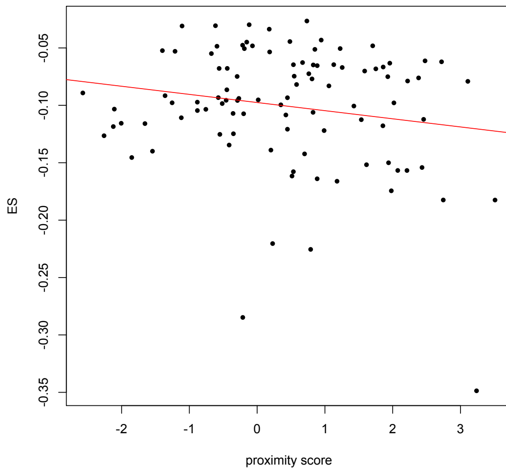
Fig S3. Scatter plot showing the relationship between enrichment score and proximity score. No significant correlation was observed between ES and proximity score (Spearman's correlation coefficient = -0.08, P = 0.407)
