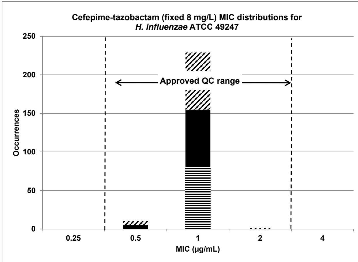
Figure S7 Cefepime-tazobactam (fixed 8 mg/L) MIC distributions for H. influenzae (ATCC 49247) by the broth microdilution testing method
