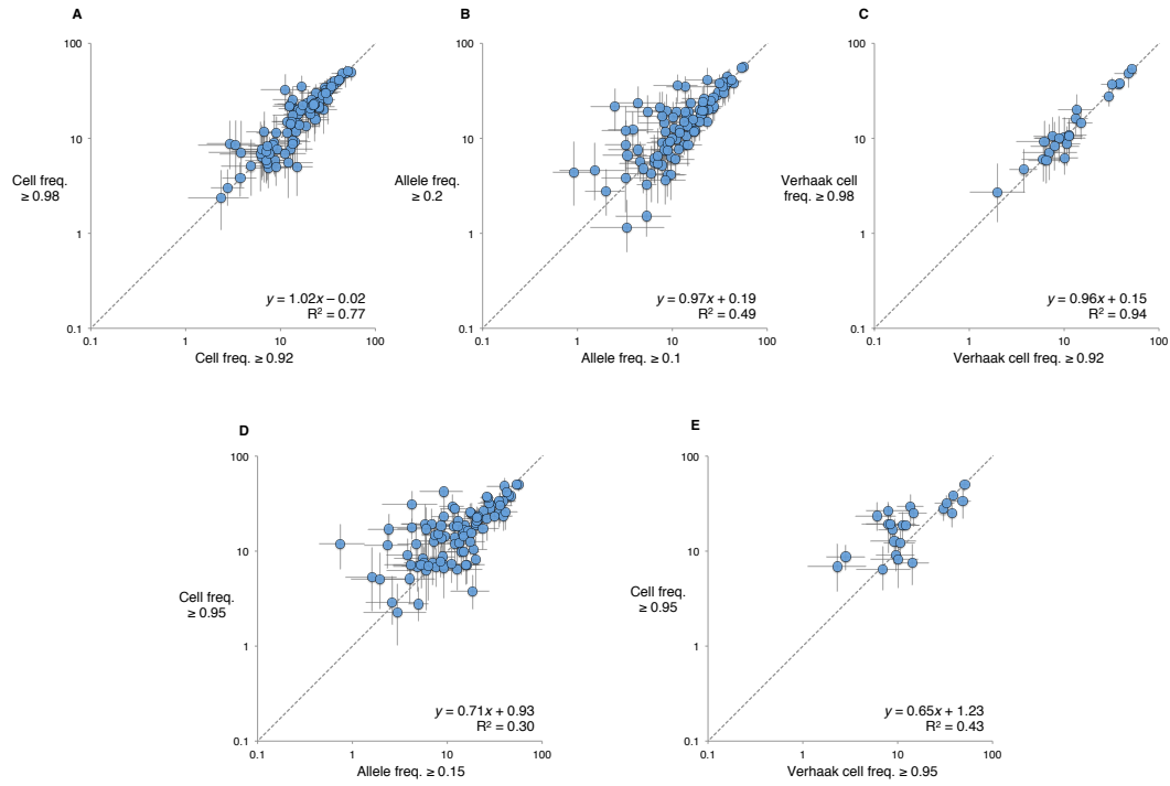
Additional Figure M5. Sensitivity analysis for time between lineage divergence and diagnosis, using a variety of clonality cutoffs. Each panel shows per-patient comparisons of the estimated time prior to diagnosis that the initial and recurrent lineages diverged, in years, for two different clonality cutoffs. All panels and legend as in Additional Figure M3.
