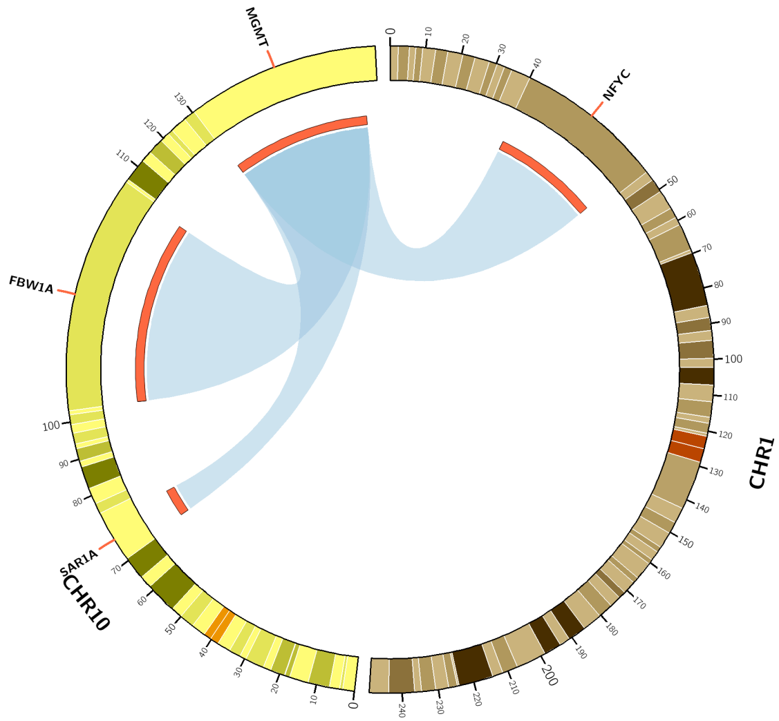
Supplementary Figure 4: Circos plot of MGMT fusions.
