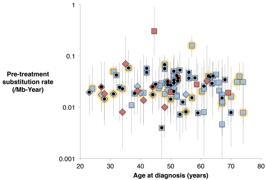
Supplementary Figure 8: No relationship is evident between pre-treatment substitution rate and age at diagnosis (median and 95% credible interval shown for each patient). Symbol legend as in Figure 3C,D.
