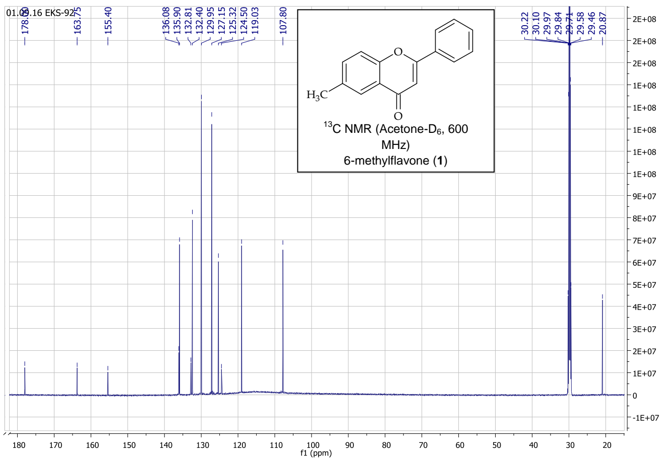
S3 Fig. 13 C NMR spectrum of 6-methylflavone (1) (Acetone-D 6 , 600 MHz).
