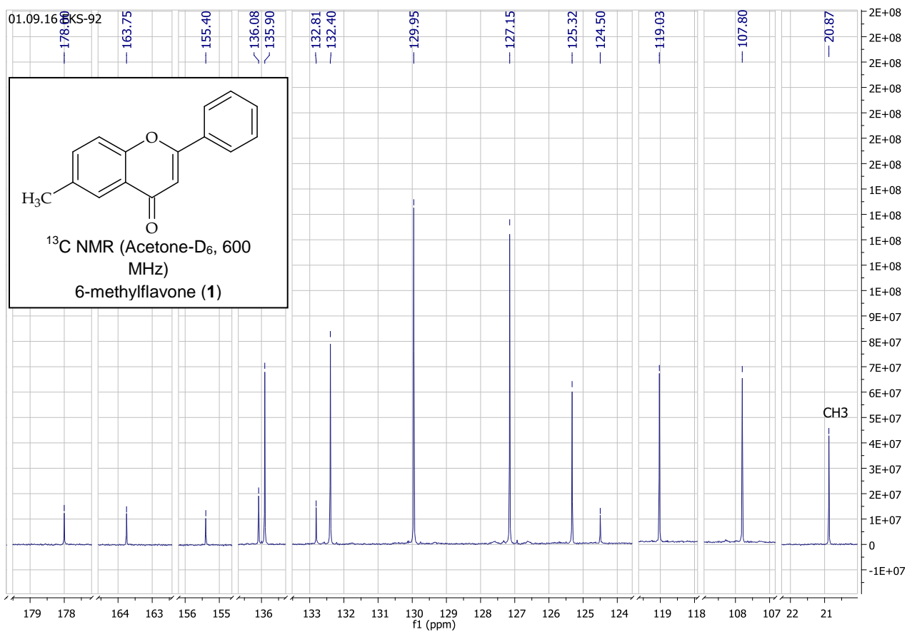
S4 Fig. 13 C NMR spectrum of 6-methylflavone (1) (Acetone-D 6 , 600 MHz).
