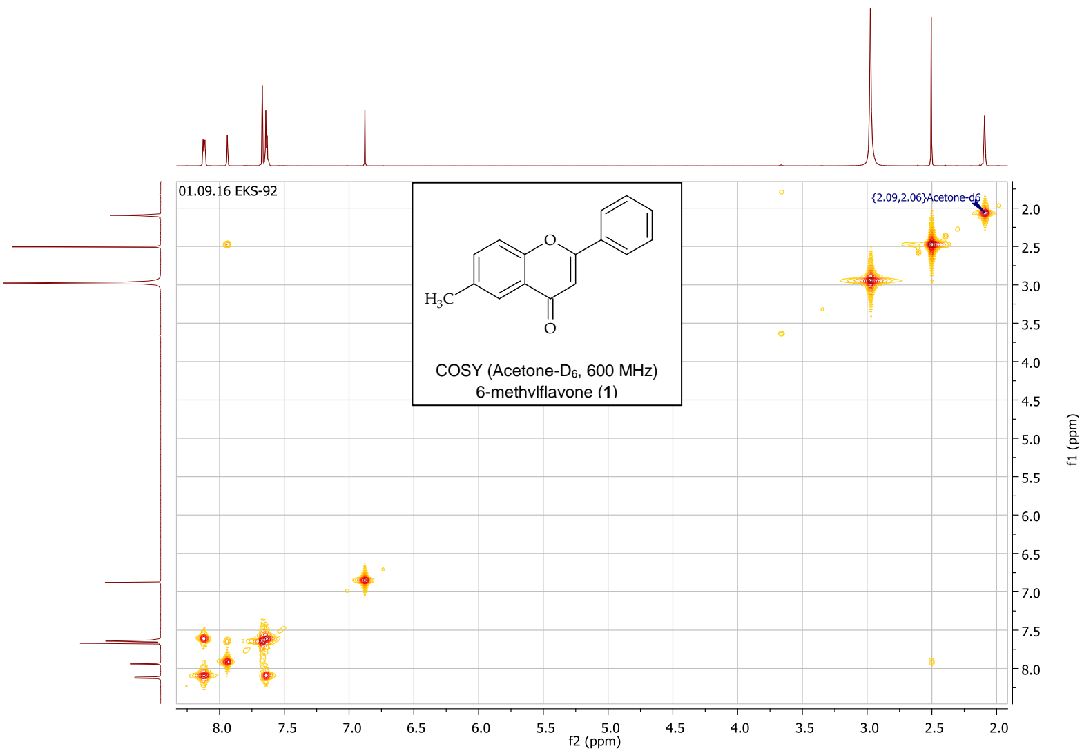
S5 Fig. COSY NMR spectrum of 6-methylflavone (1) (Acetone-D 6 , 600 MHz).
