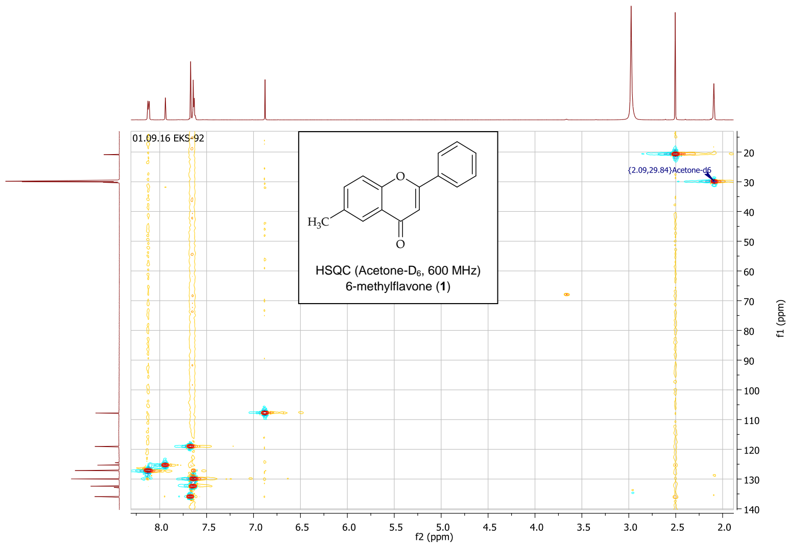
S6 Fig. HSQC NMR spectrum of 6-methylflavone (1) (Acetone-D 6 , 600 MHz).
