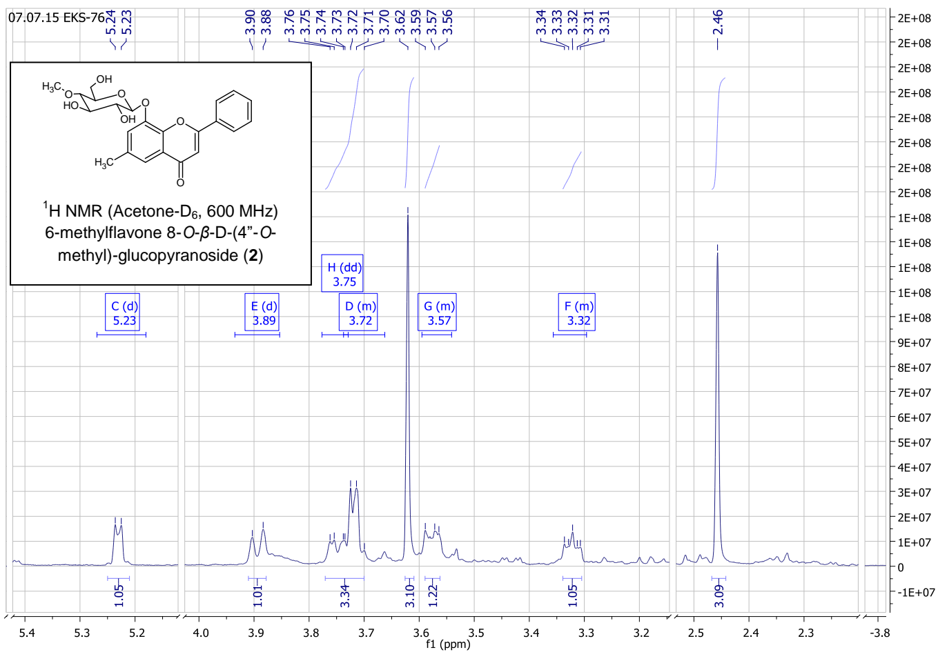
S9 Fig. 1 H NMR of 6-methylflavone 8-O-β-D-(4''-O-methyl)-glucopyranoside (2) (Acetone-D 6 , 600 MHz).
