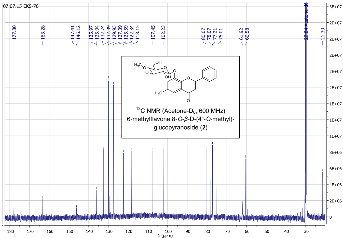
S10 Fig. 13 C NMR of 6-methylflavone 8-O-β-D-(4''-O-methyl)-glucopyranoside (2) (Acetone-D 6 , 600 MHz).
