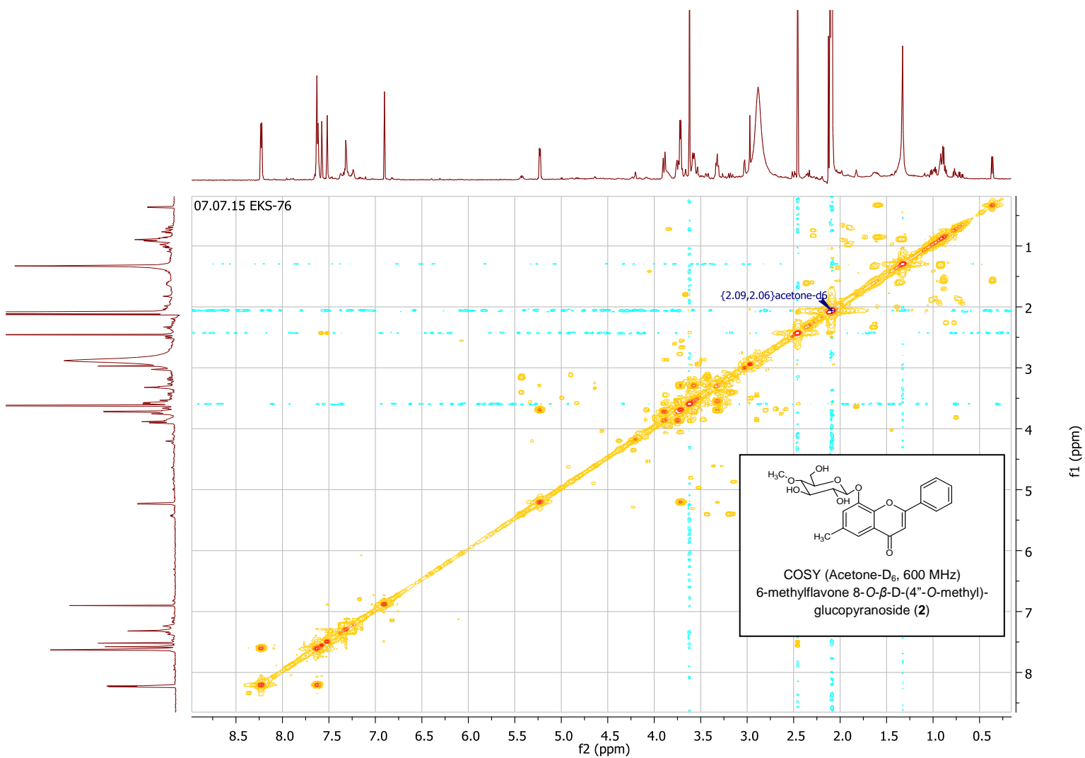
S11 Fig. COSY NMR of 6-methylflavone 8-O-β-D-(4''-O-methyl)-glucopyranoside (2) (Acetone-D 6 , 600 MHz).
