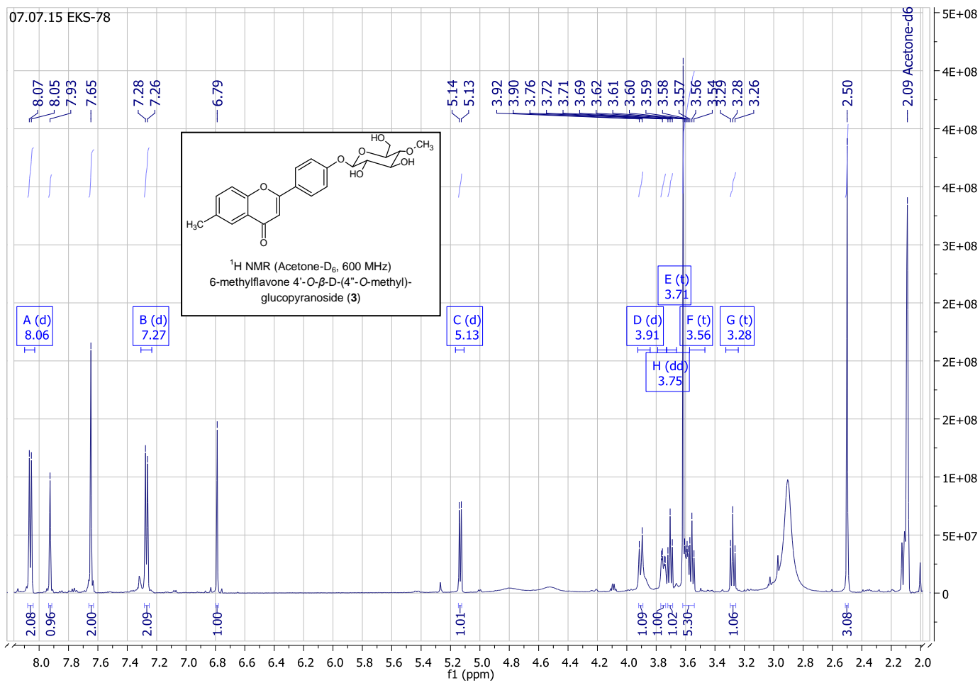
S14 Fig. 1 H NMR of 6-methylflavone 4'-O-β-D-(4''-O-methyl)-glucopyranoside (3) (Acetone-D 6 , 600 MHz).
