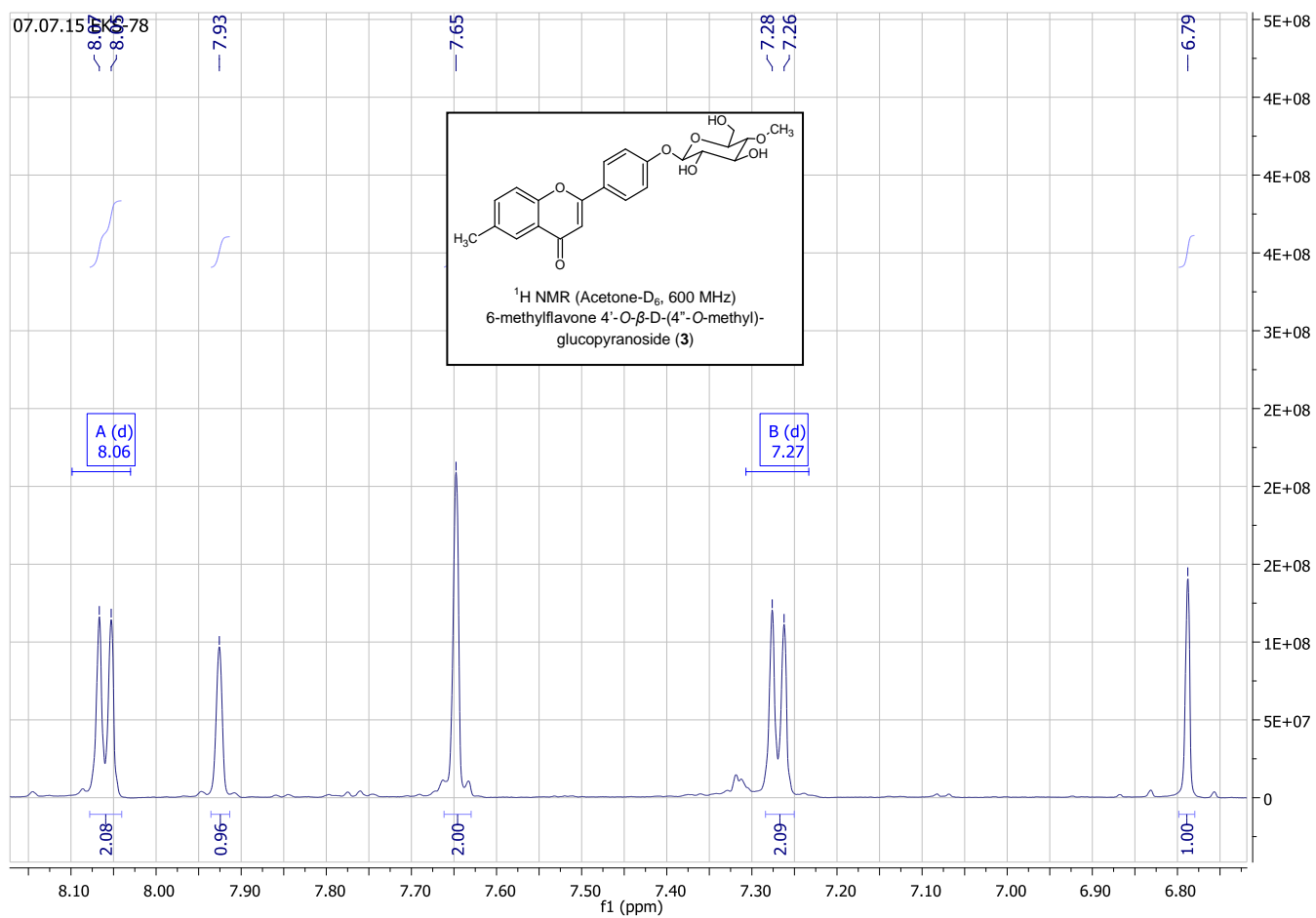
S15 Fig. 1 H NMR of 6-methylflavone 4'-O-β-D-(4''-O-methyl)-glucopyranoside (3) (Acetone-D 6 , 600 MHz).
