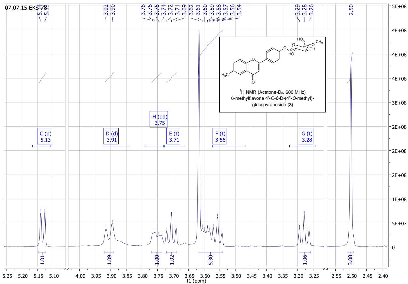
S16 Fig. 1 H NMR of 6-methylflavone 4'-O-β-D-(4''-O-methyl)-glucopyranoside (3) (Acetone-D 6 , 600 MHz).
