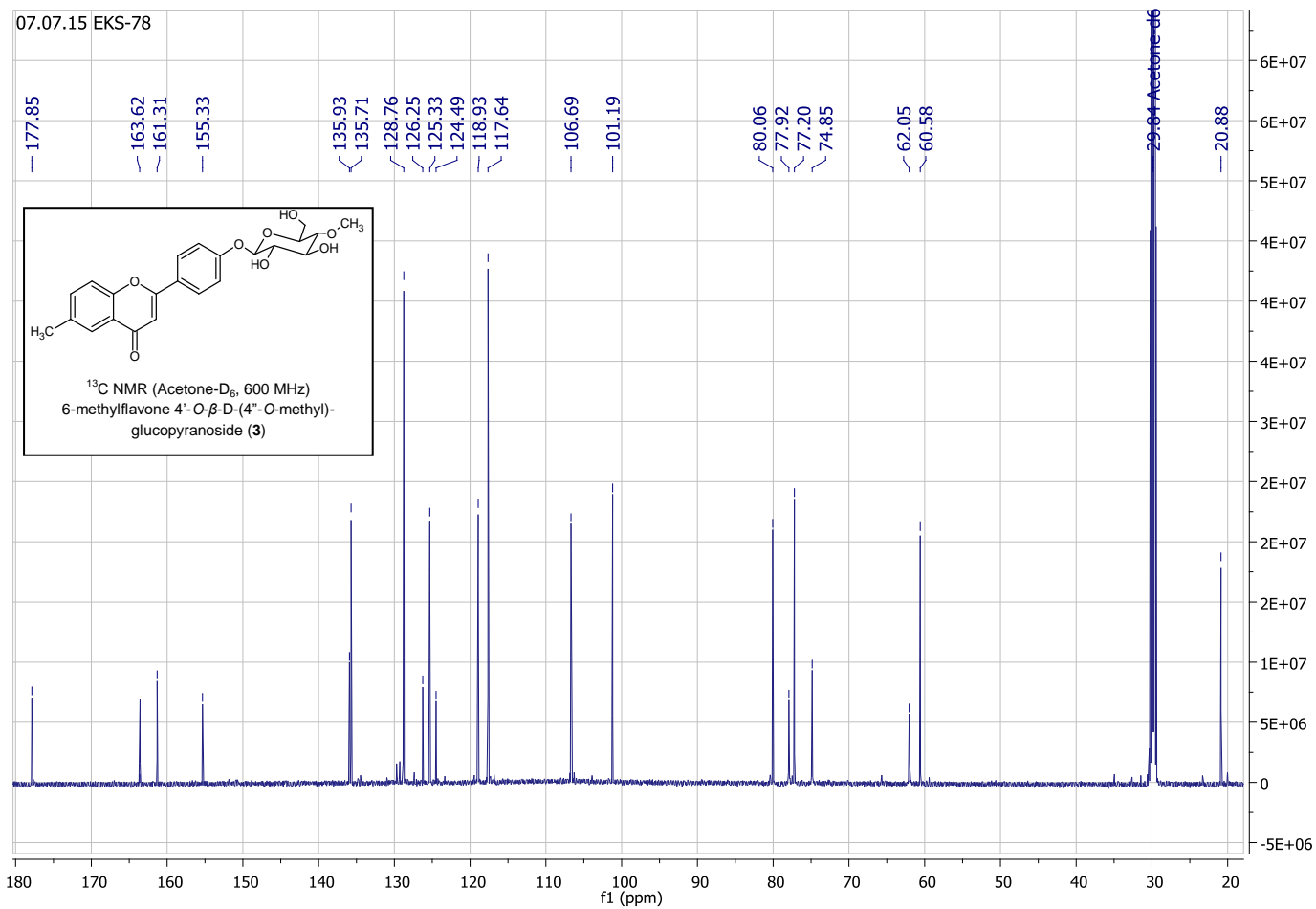
S17 Fig. 13 C NMR of 6-methylflavone 4'-O-β-D-(4''-O-methyl)-glucopyranoside (3) (Acetone-D 6 , 600 MHz).
