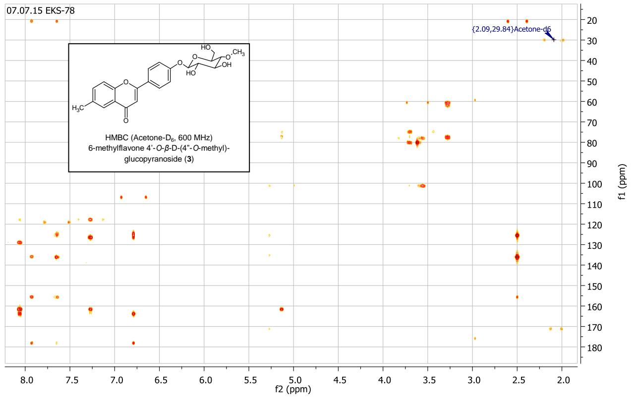
S20 Fig. HMBC NMR of 6-methylflavone 4'-O-β-D-(4''-O-methyl)-glucopyranoside (3) (Acetone-D 6 , 600 MHz).
