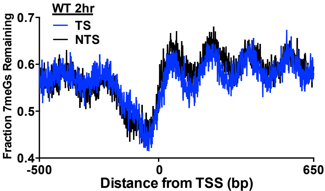
Supplemental Figure S2. Repair of 7meG lesions shows no obvious strand bias among yeast genes in WT cells. Fraction of 7meG lesions remaining following 2hr repair in WT cells relative to a matched 0hr mag1 \Delta control. Data is shown for DNA regions surrounding the transcription start site (TSS) of 5762 yeast genes. The transcribed strand (TS) is depicted in blue and the non-transcribed strand (NTS) is depicted in black.
