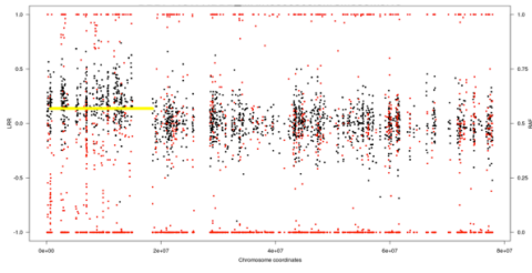
SNP blood
