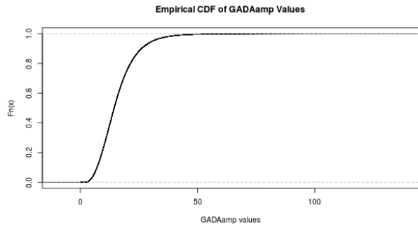
Supplementary Figure 23: Distribution of size and signal-strength of false positives: The histograms of probe-number and GADAamp values both show long tails, with the majority of putative events being smaller and weak. We plotted the cumulative distribution functions from the data and showed that events with greater than about 100 probes or about 25 GADAamp were very rare in the false positive events.
