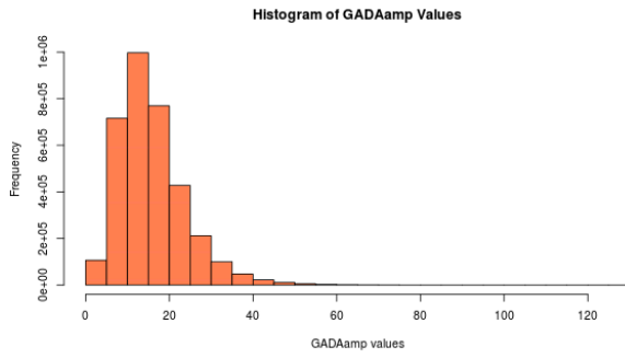
Supplementary Figure 23: Distribution of size and signal-strength of false positives: The histograms of probe-number and GADAamp values both show long tails, with the majority of putative events being smaller and weak. We plotted the cumulative distribution functions from the data and showed that events with greater than about 100 probes or about 25 GADAamp were very rare in the false positive events.
