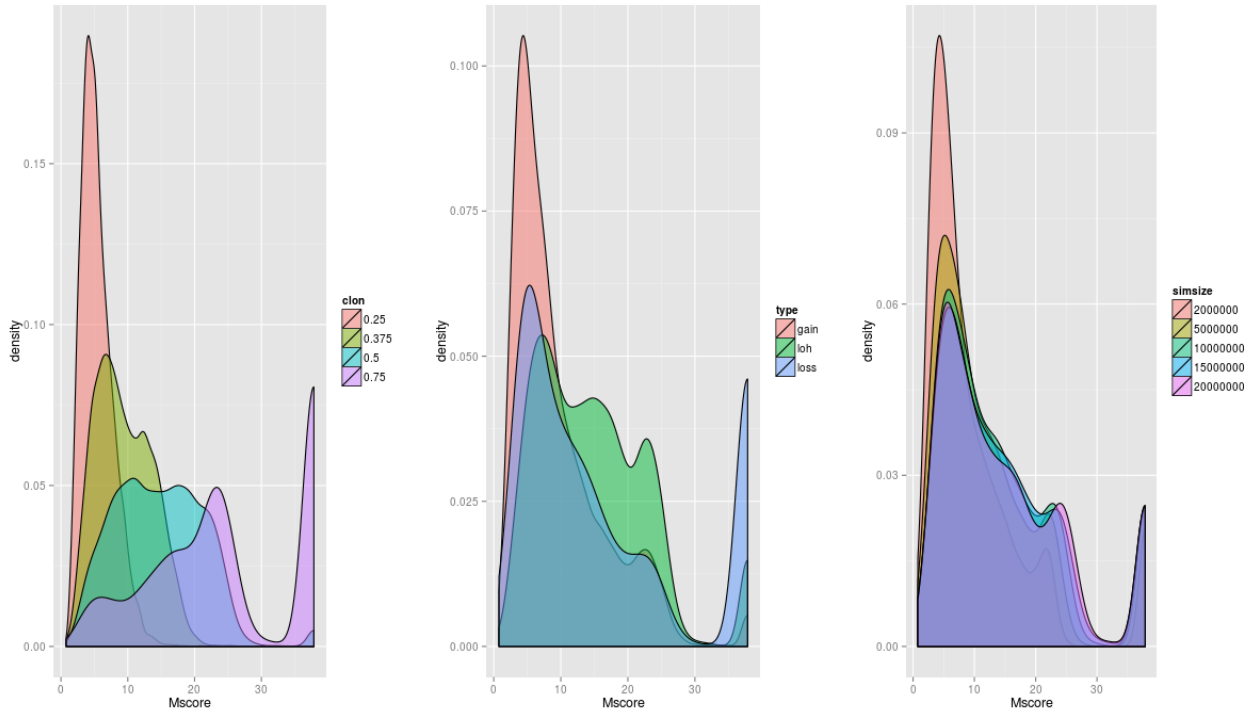
Supplementary Figure 25: Stratifying Mscore by simulation clonality, type, and size: We stratified the true positive events by Mscore to better define the relationship between Mscore thresholds and simulated mosaic events. The mosaic events with the lowest Mscore were those at the lowest clonality (left side of left graph).
