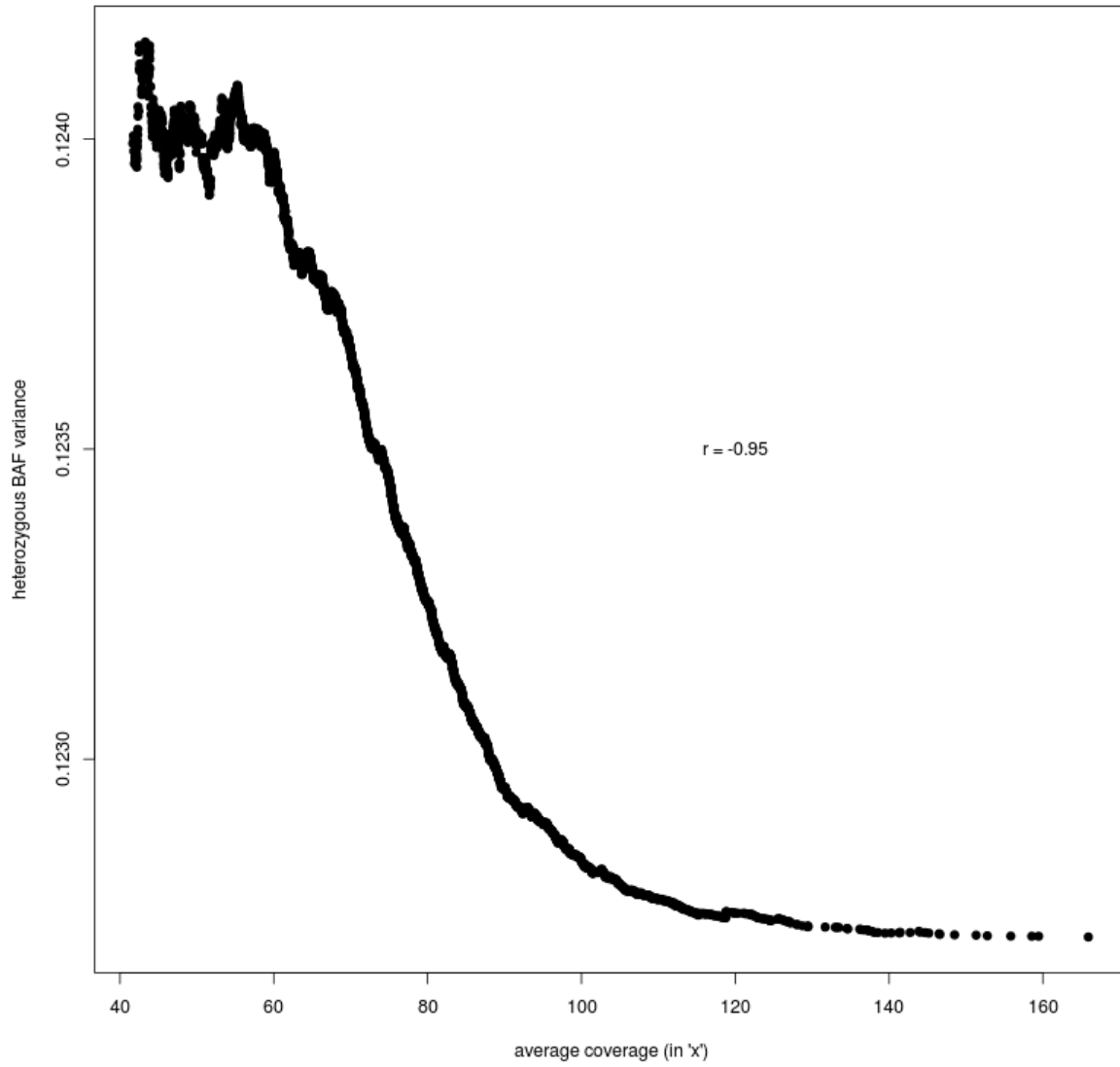
Supplementary Figure 7: The effect of average coverage on BAF variance.
