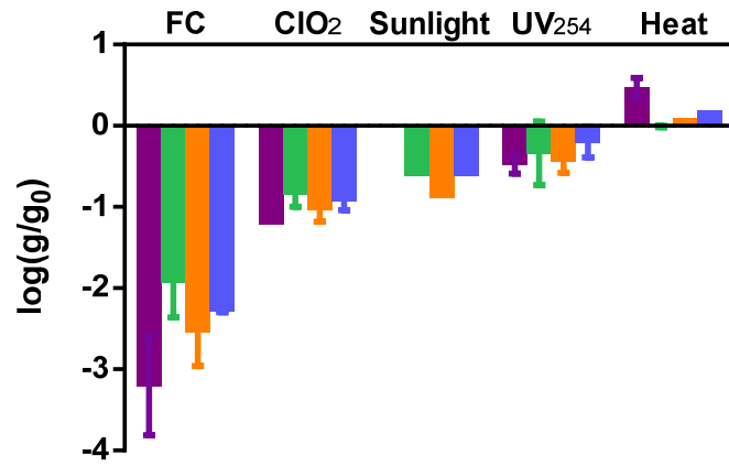
Supplementary Figure 2. Decay of four genome segments ( \log(g/g_0) ) upon inactivation by FC, ClO 2 , sunlight, UV 254 and heat. Segment 1 was not tested for decay by sunlight. Error bars represent the standard deviation of triplicate experiments.
