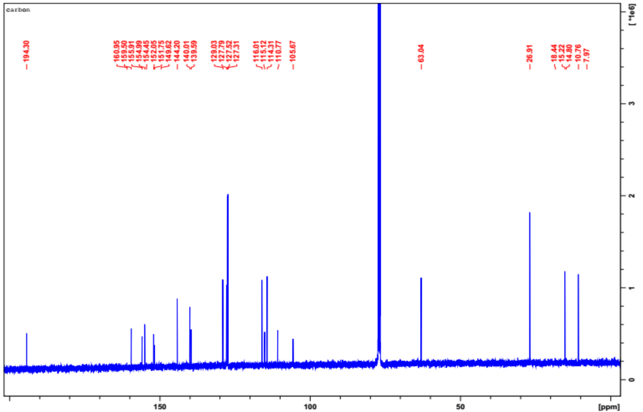
S2 Fig. ^{13}\text{C} -NMR analysis of isolated calophyllolide (CP)
