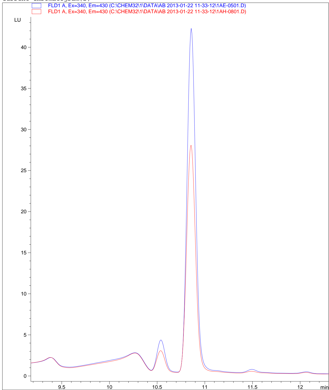
Current Chromatogram(s)
