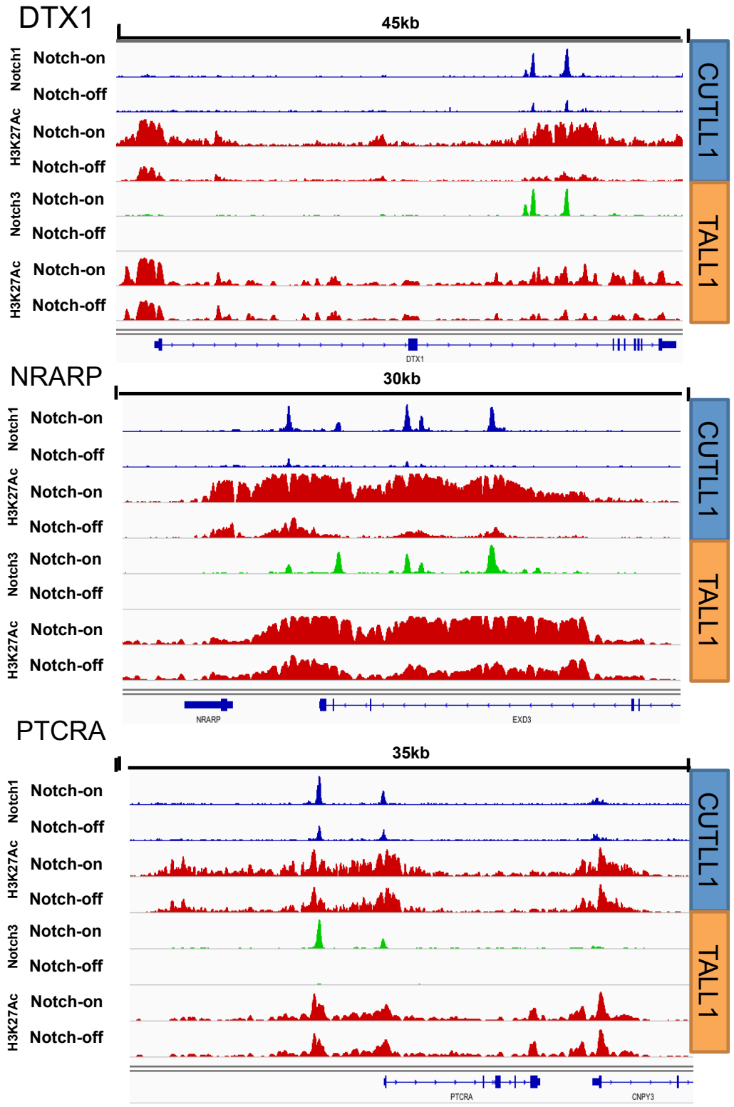
Supplemental Figure 2. IGV tracks showing similar chromatin and Notch-binding chromatin landscapes near DTX1 , NRARP , and PTCRA in TALL1 and CUTLL1 cells.
