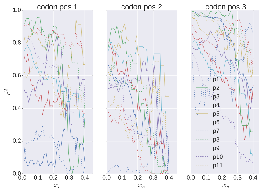
Fig S4. Coefficient of determination for average pairwise distance (diversity), by codon position. (Genetic region: pol .)
