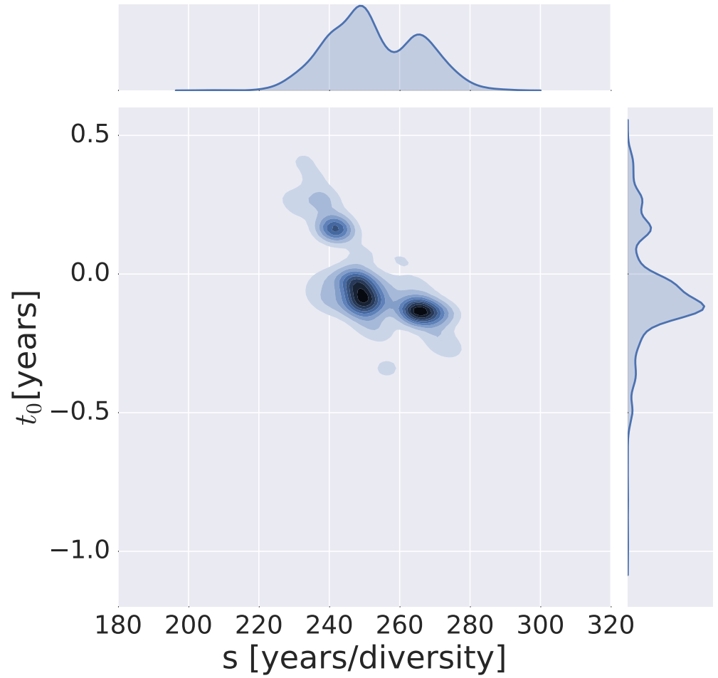
Fig S6. Distribution of slopes ( s ) and intercepts ( t_0 ) (bootstrapped over the patients of the training dataset). (Genetic region: 3rd codon positions in pol , diversity measure: average pairwise distance, x_c = 0.003 .)
