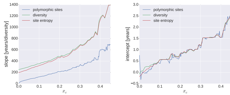
Fig S7. Dependence of the slope and intercept in the cutoff. (Genetic region: 3rd codon positions in pol , diversity measure: average pairwise distance.)
