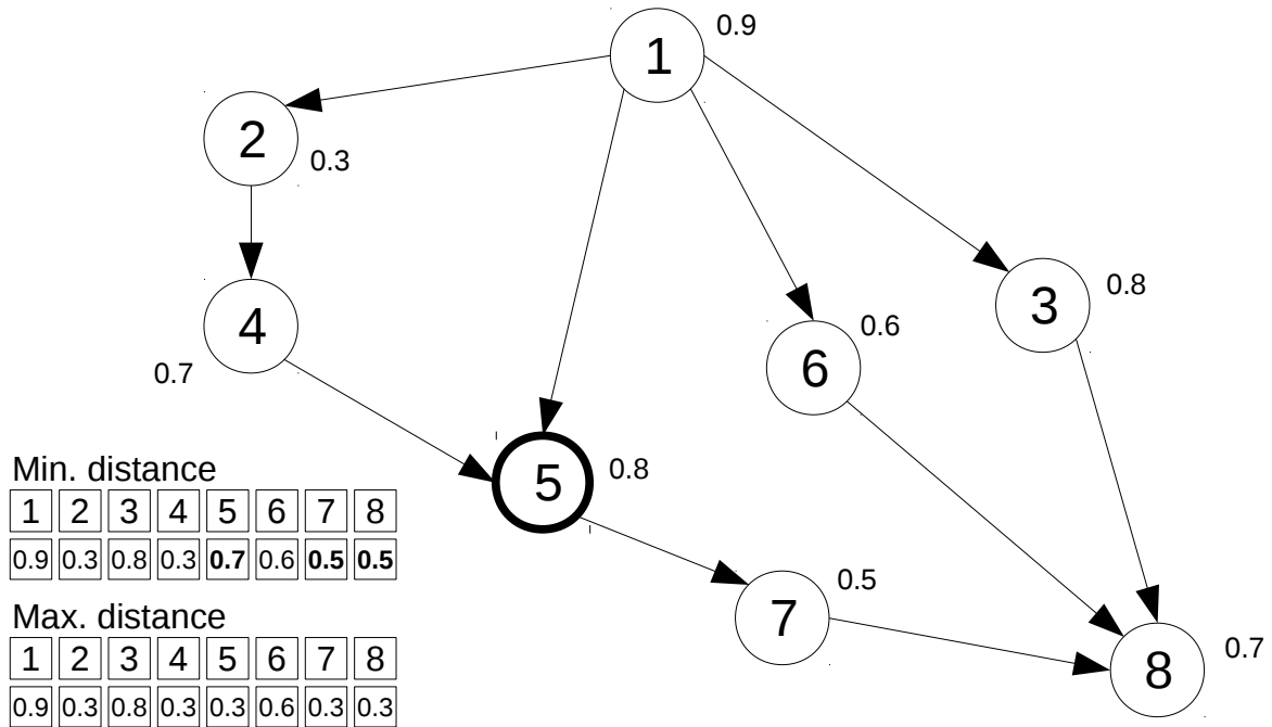
Additional Figure 2: Levels defined in terms of the minimum distance from the root (node 1) lead to inconsistent predictions. The small numbers close to nodes correspond to the \hat{y}_i scores of the flat predictions. The Hierarchical top-down scores obtained respectively by crossing the levels according to the minimum and the maximum distance from the root are shown in the bottom-left. Scores in boldface represent inconsistent predictions.
