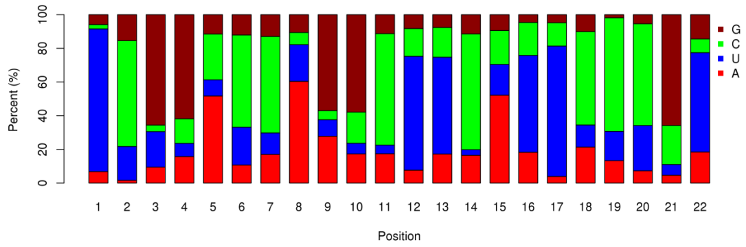
miRNA Nucleotide Bias at Each Position (VMS)
