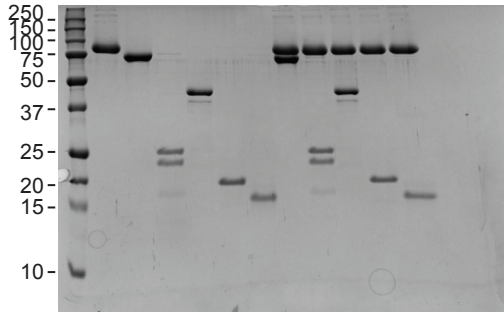
Figure 5E_Input
