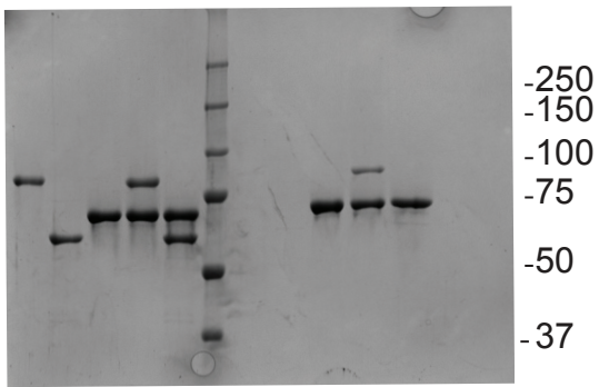
Figure 5B_Input / His-Pulldown
