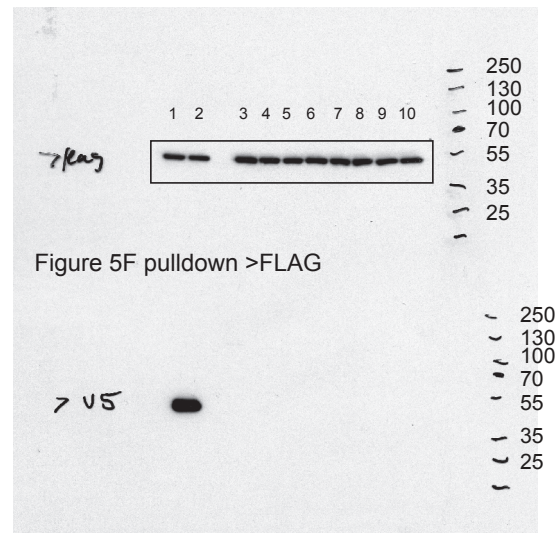
Figure 5F_pulldown >FLAG
