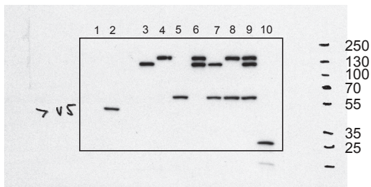
Figure 5F_input >V5
