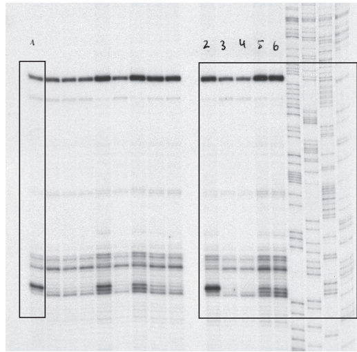
Figure 5G
