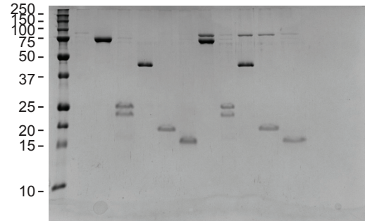
Figure 5E_His-Pulldown
