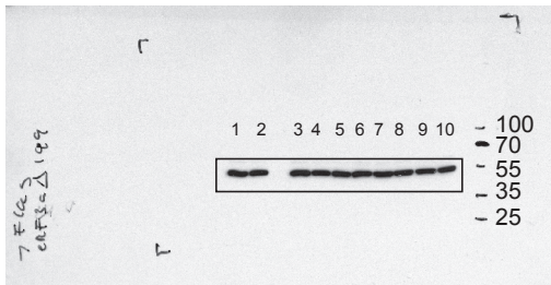
Figure 5F_input >FLAG
