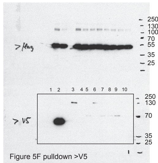
Figure 5F_pulldown >V5
