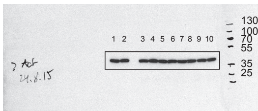
Figure 5F_input >ACTB
