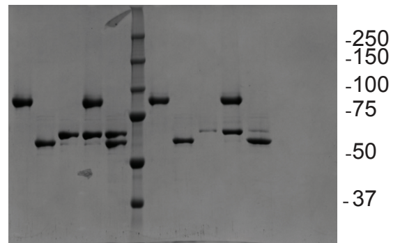
Figure 5C_Input / His-Pulldown
