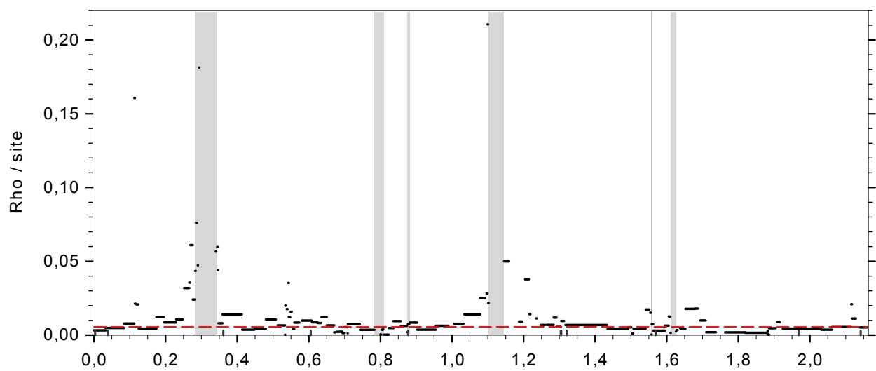
Genome position on QLW-P1DMWA-1 (Mbp)
