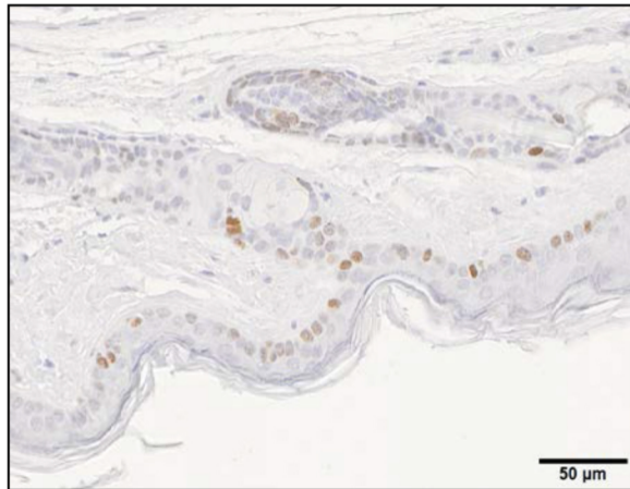
Ki67 Positive control
