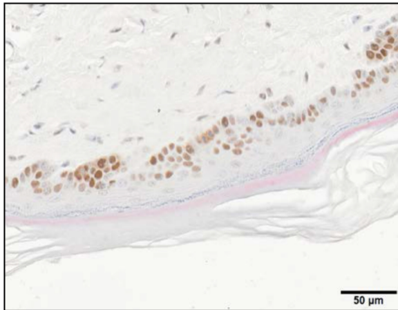
PCNA Positive control
