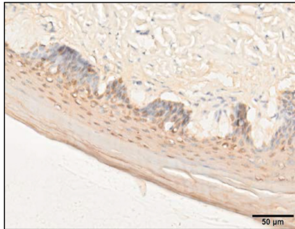
BrdU Positive control
