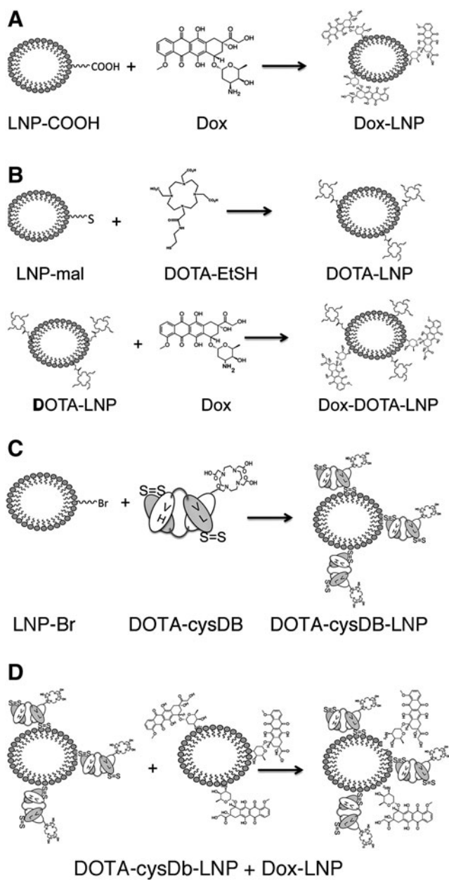
SUPPLEMENTARY FIG. S2. Schematic diagram depicting assembly of nanoparticle constructs. (A) Dox-LNP. (B) Dox-DOTA-LNP. (C) DOTA-cys-DB-LNP. (D) Mixing of DOTA-cys-DB-LNP and Dox-DOTA-LNP. cys-DB, cys-diabody; Dox, doxorubicin; LNP, lipid nanoparticle.
