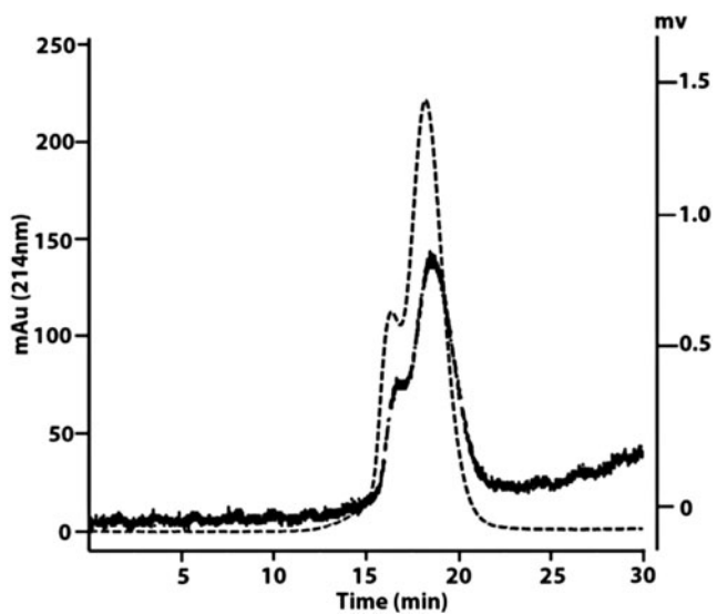
SUPPLEMENTARY FIG. S4. SEC analysis of Dox-DOTA-LNP. The Dox-DOTA-LNP was analyzed on SEC by Absorbance 214 ( solid line ) and fluorescence ( dashed line ) revealing two poorly separated peaks, eluting at 16 and 18 minutes. Dox, doxorubicin; LNP, lipid nanoparticle; SEC, size-exclusion chromatography.
