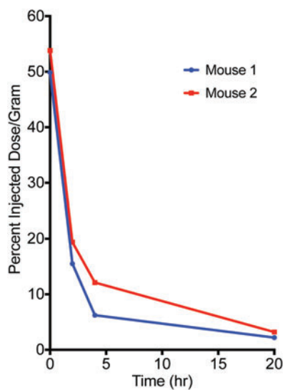
SUPPLEMENTARY FIG. S5. Blood clearance of ^{64}\text{Cu} -Dox-DOTA-LNP. The ^{64}\text{Cu} -Dox-DOTA-LNP was injected into two NOD/SCID mice, and blood was collected at various times, counted for radioactivity. The data are plotted as percent injected dose per gram versus time to show the clearance rate. Dox, doxorubicin; NOD/SCID, non-obese diabetic severe combined immune deficiency; LNP, lipid nanoparticle.
