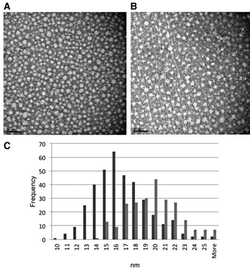
SUPPLEMENTARY FIG. S6. EM analysis of DOTA-cys-DB-LNP mixed with Dox-LNP. (A) The Dox-LNP was mounted on an EM grid, stained with uranyl acetate and analyzed by TEM. (B) DOTA-cys-DB-LNP + Dox-LNP mixture was analyzed by TEM. (C) Size comparison of the Dox-LNP micelles ( blue bars ) increased from 16 nm to 20 nm for the DOTA-cys-DB-LNP + Dox-LNP mixture ( rust bars ). cys-DB, cys-diabody; Dox, doxorubicin; EM, electron microscopy; LNP, lipid nanoparticle; TEM, transmission electron microscopy.
