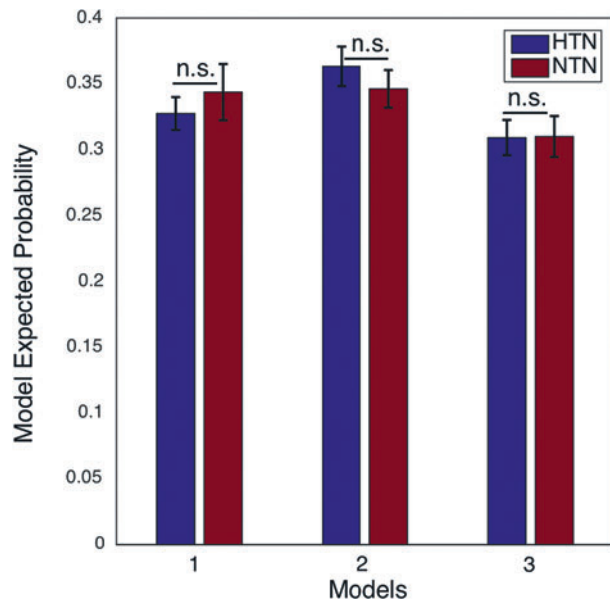
SUPPLEMENTARY FIG. S2. Comparison of model expected probability value using random effects analysis between HTN and NTN cognitively normal individuals within each model demonstrating n.s. statistical difference ( t -test; p > 0.3 ). HTN, hypertensive; n.s., not significant; NTN, normotensive.
