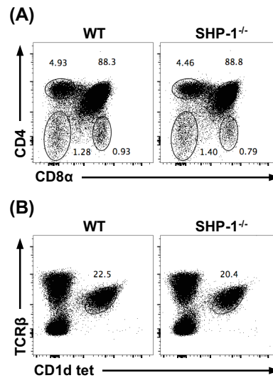
Supplementary Figure 3. SHP-1 is dispensable for T and iNKT cell development. (A) Representative FACS plots show thymic T cell development in SHP-1 fl/+ -CD4Cre (WT) and SHP-1 fl/fl -CD4Cre (SHP-1 -/- ) mice. (B) Representative FACS plots show hepatic iNKT cells in WT and SHP-1 -/- mice. Data are representative of at least two independent experiments, n = 9 Het and n=8 KO mice.
