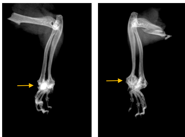
Supplementary Figure 5. Adult SHP-2 -/- CD4-Cre RAG1 -/- mice develop cartilage tumors. Representative Faxitron X-ray of euthanized mice. Arrows highlight the location of the cartilage tumors on wrists. Analysis was performed on 3 SHP-2 -/- RAG1 -/- CD4-Cre mice and controls.
