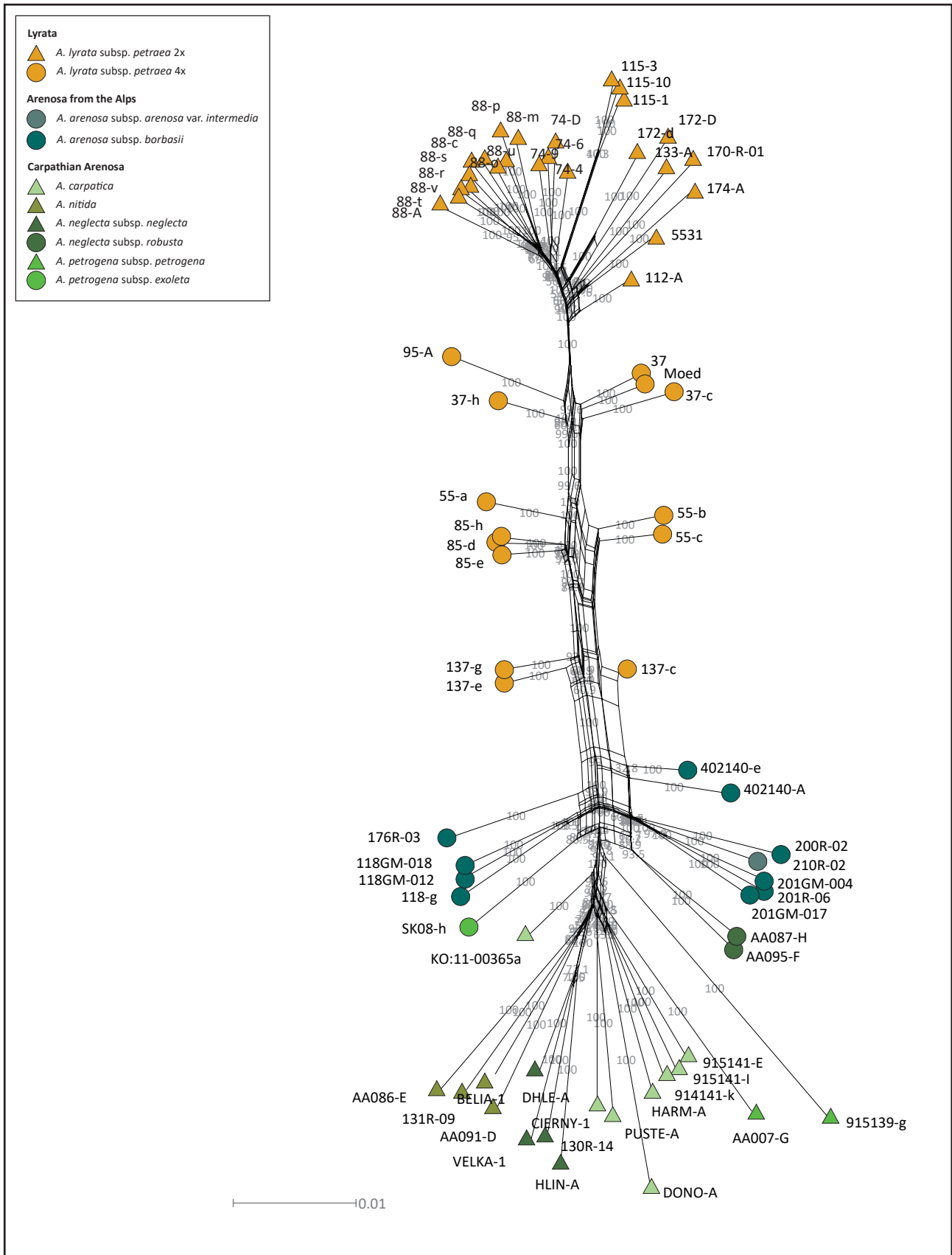
Additional File 1. SplitsTree [47] equal angle NeighborNet based on 5,473,967 SNPs from the nuclear genome. Bootstrap values from 1000 replicates are indicated in grey. Taxa are indicated with color codes, diploids are shown with triangles and tetraploids with circles.
