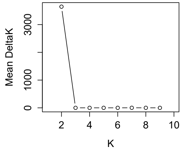
Additional File 6. Structure-sum [85] output, analysis of deltaK and similarity values between 10 independent STRUCTURE [45,82] runs.
