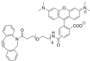
aza-dibenzocyclooctyne- carboxytetramethylrhodamine (DBCO-TAMRA)
