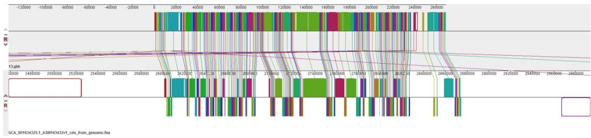
2 Fig. S1 Alignment of contig 13 in A. veronii 172 with the complete chromosome of A. 3 veronii (GenBank accession no. CP014774.1). Block outlines with the same color 4 represent homologous regions, which are connected by lines. Areas outside the block 5 are the regions that do not match. The scale plate above the block indicates the length 6 of the contig.
