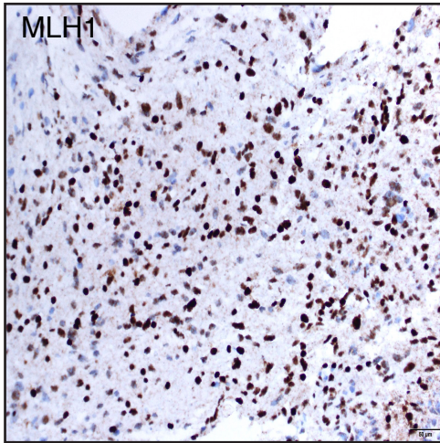
Supplementary Figure S3. Immunohistochemical staining for the MMR panel (MLH1, MSH2, MSH6, PMS2) in the HGG11 primary tumor.
