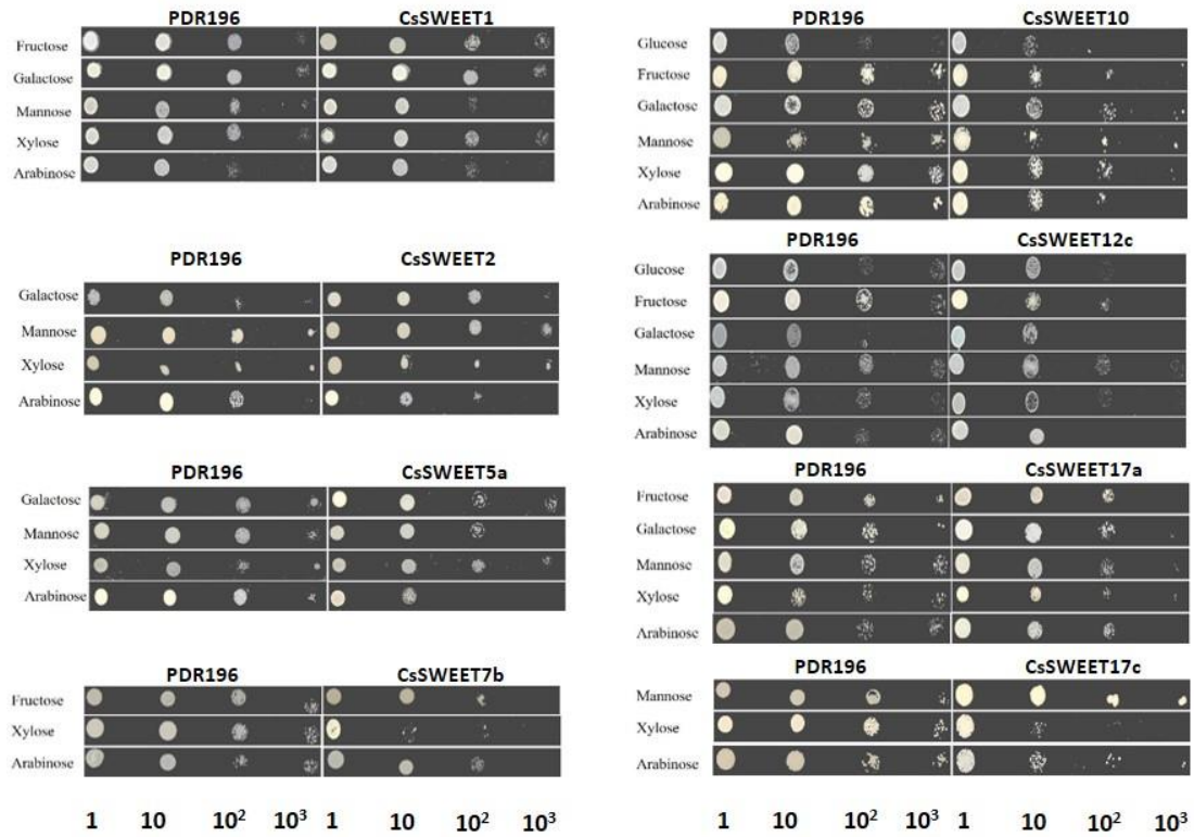
Fig. S2. Heterologous expression of eight CsSWEET genes in hexose uptake-deficient yeast strain EBY.VW4000. No obviously uptake were observed in recombinant vectors or the empty pDR196 vector (as a negative control) when grew on SD (synthetic deficient)-ura medium supplemented with 2% sugar (listed above) as the sole carbon.
