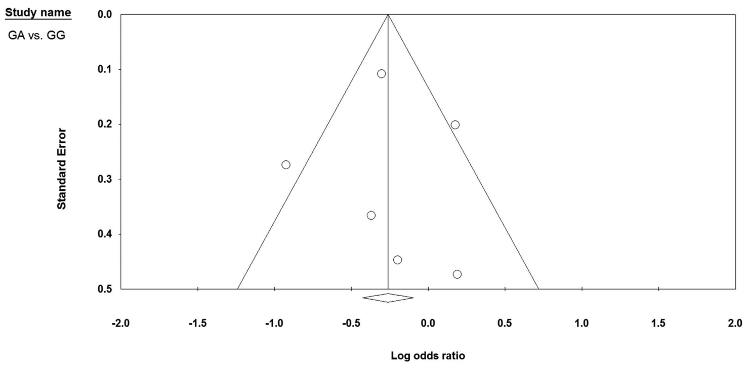
Funnel Plot of Standard Error by Log odds ratio
